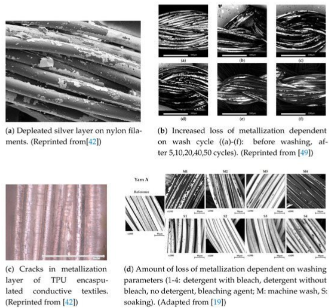
Figure 2. Examples of loss of metallization after washing.
