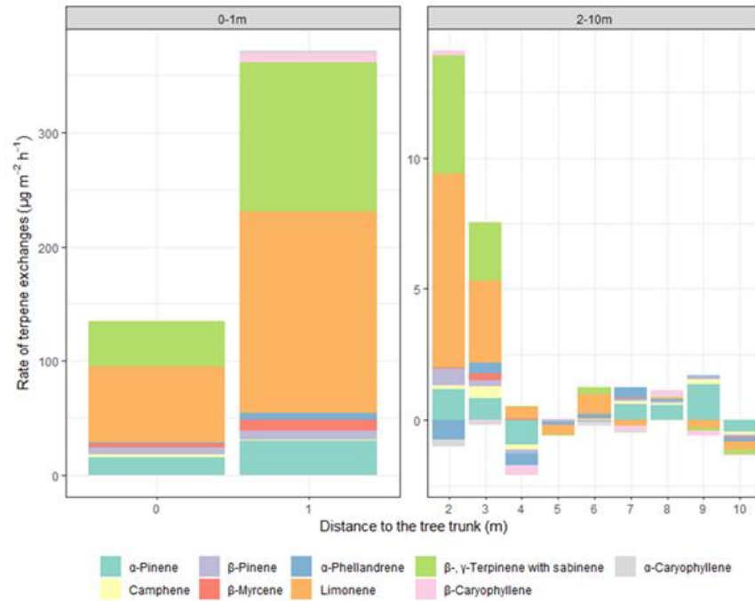
Figure 2. Distribution of terpene exchange along the transects.
