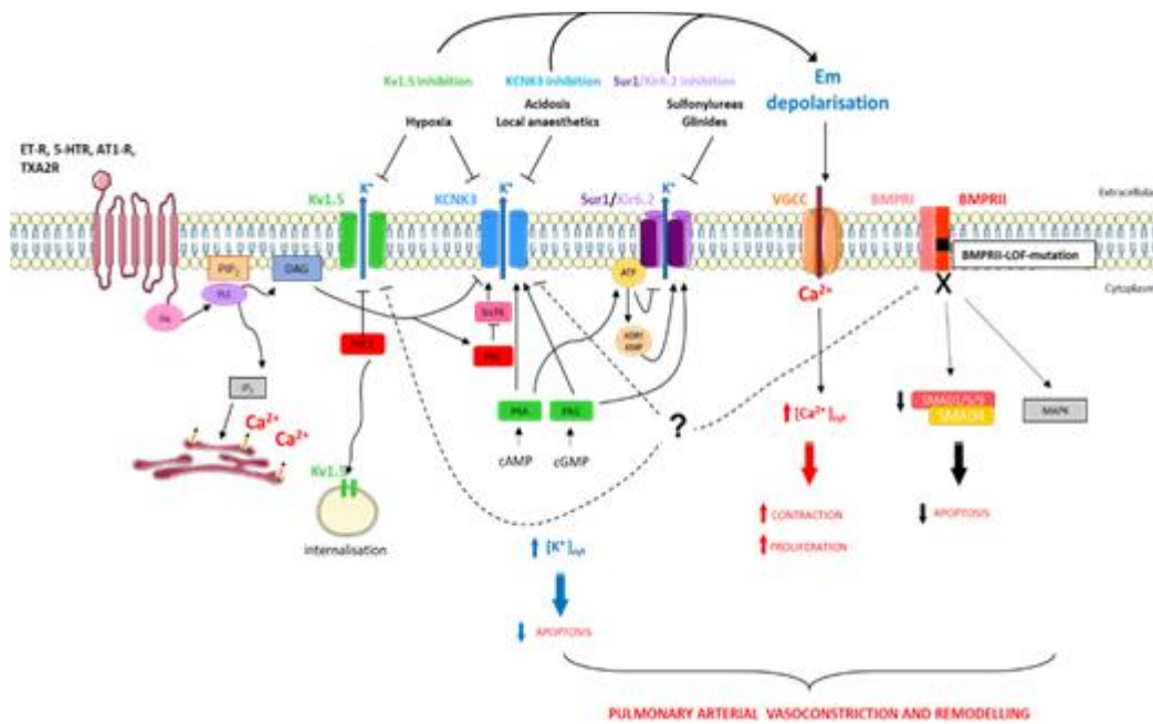
Figure 2. Schematic representation of pathways implicated in K + regulation in pulmonary artery smooth muscle cells in the context of pulmonary arterial hypertension (PAH). [Ca 2+ ] cyt , cytoplasmic calcium concentration; [K + ] cyt , cytoplasmic potassium concentration; 5-HTR, serotonin receptor; AT1-R, angiotensin 1 receptor; BMPRI, BMP receptor type I; BMPRII, BMP receptor type II; cAMP, cyclic adenosine monophosphate; cGMP, cyclic guanosine monophosphate; DAG, diacylglycerol; Em, membrane resting potential; ET-R, endothelin receptor; IP 3 , inositol-1,4,5-triphosphate; MAPK, mitogen-activated protein kinases; PIP 2 , phosphatidylinositol-4,5-bisphosphate; PKA, protein kinase A; PKC, protein kinase C; PKG, protein kinase G; PLC, phospholipase C; SMAD, mothers against decapentaplegic homologue; SrcTK, Src family tyrosine kinase; TXA 2 R, thromboxan A2 receptor.
