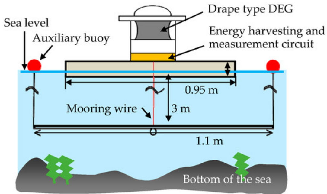
Figure 12. Buoy power generation system with plate.
