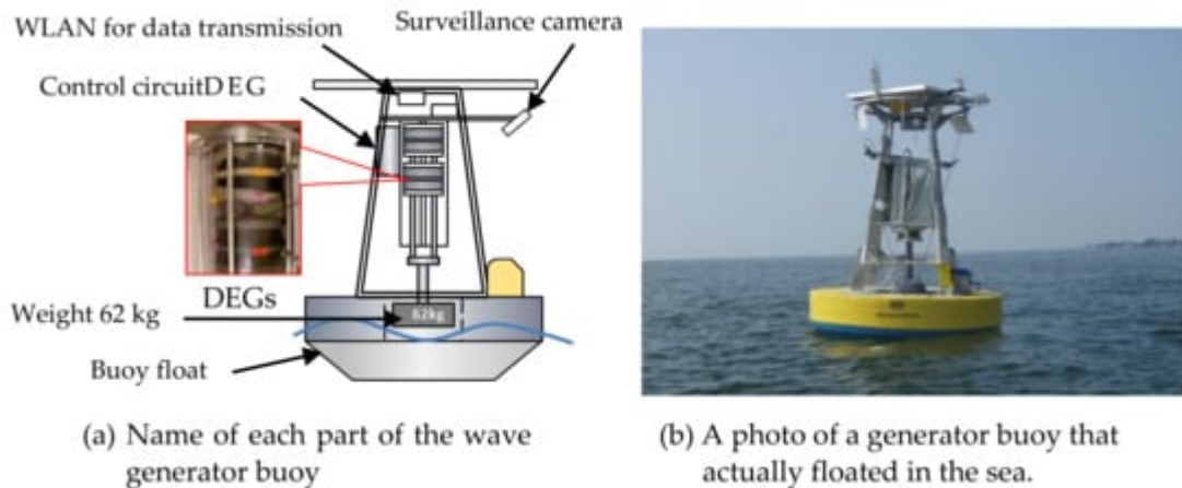
Figure 10. Buoy power generator system equipped with DEGs: (a) Name of each part of the wave generator buoy; (b) A photo of a generator buoy that actually floated in the sea.
