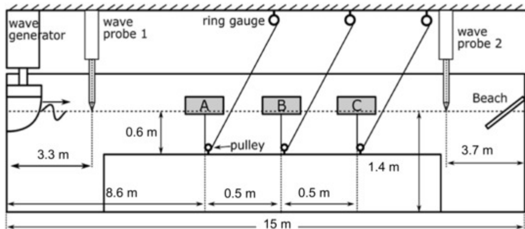
Figure 18. A test system to investigate how the waves interfere with each of the three buoys.
