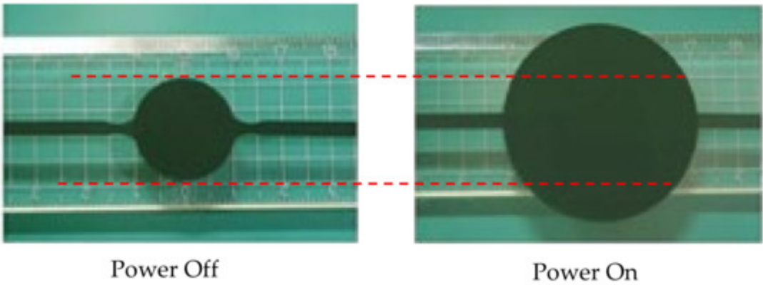
Figure 3. Expanding circular actuator up to 680%.
