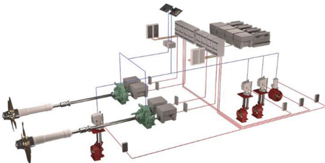
Figure 3. Typical setup of a diesel/gas electric battery hybrid propulsion system [5].
