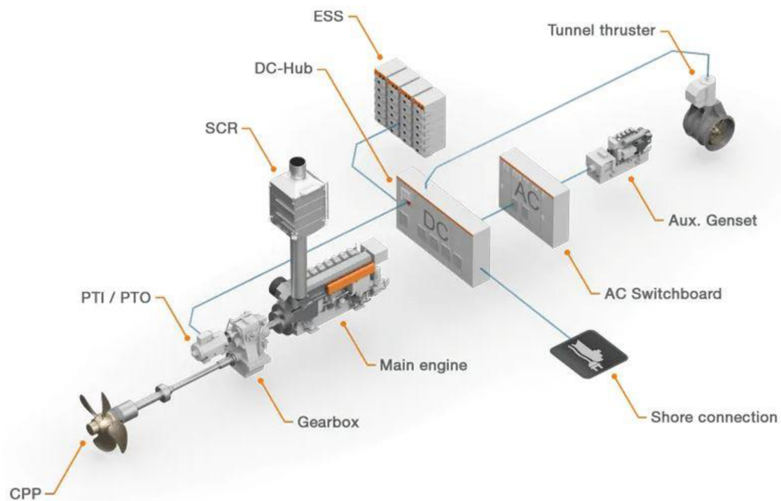
Figure 16. Hybridised CPP arrangement for short sea shipping [40] .
