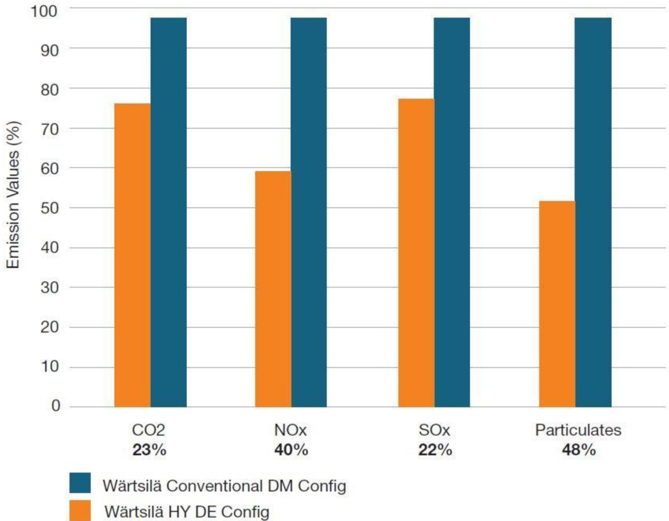
Figure 13. Emission comparison of different tug propulsion systems [27].
