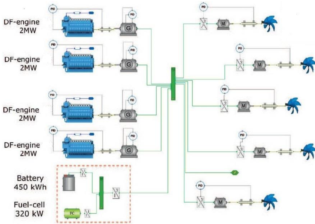
Figure 2. Battery-hybrid propulsion system on board the Viking Lady [2].
