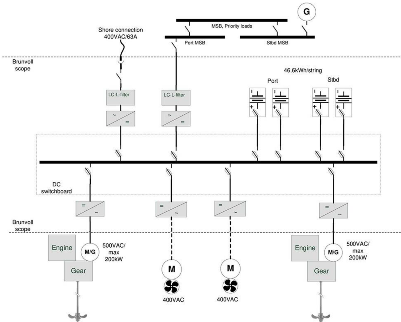
Figure 8. Single-line diagram of the high-speed vessel's propulsion system [17].
