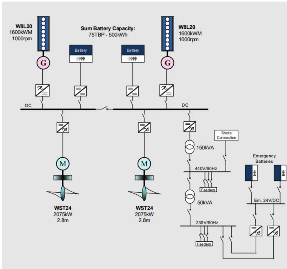
Figure 11. Single-line diagram of the diesel–electric hybrid system [28].
