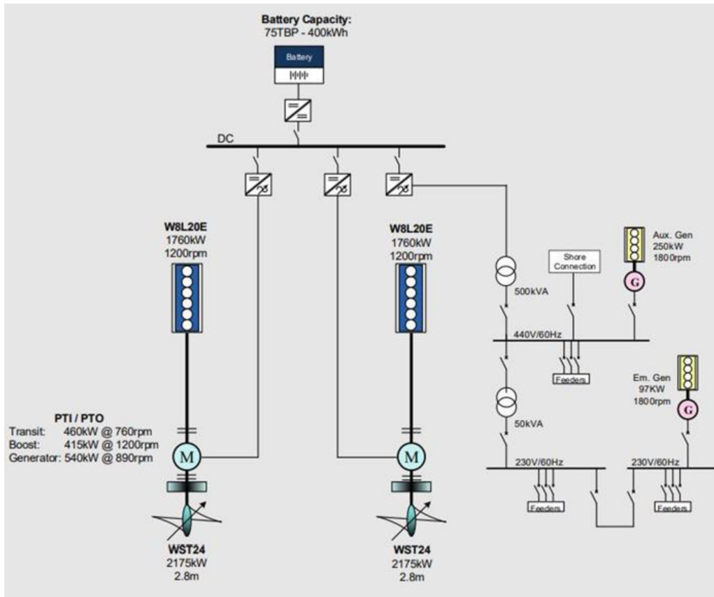
Figure 10. Single-line diagram of the diesel–mechanic hybrid system [28].
