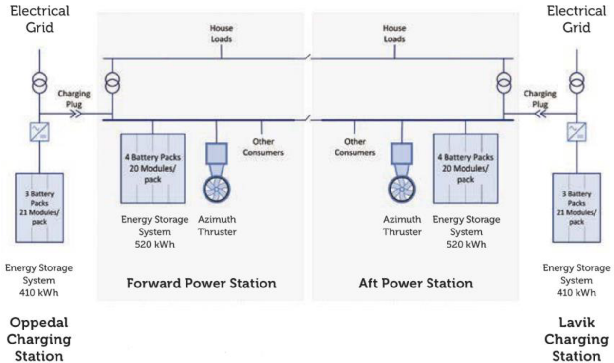
Figure 5. MF Ampere—single line diagram [10].
