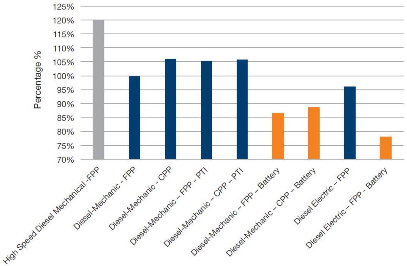
Figure 12. Fuel consumption comparison of different tug propulsion systems [27] .
