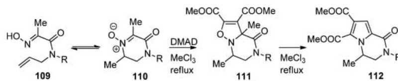
Scheme 30. Synthesis and rearrangement of isoxazolinopyrazinones.
