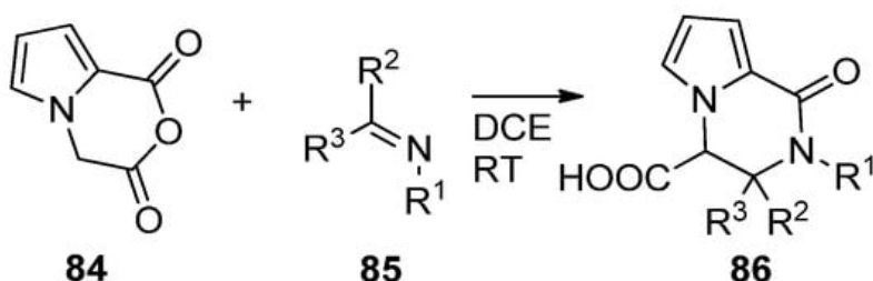
Scheme 23. Castagnoli–Cushman reaction of pyrrole cyclic anhydrides.
