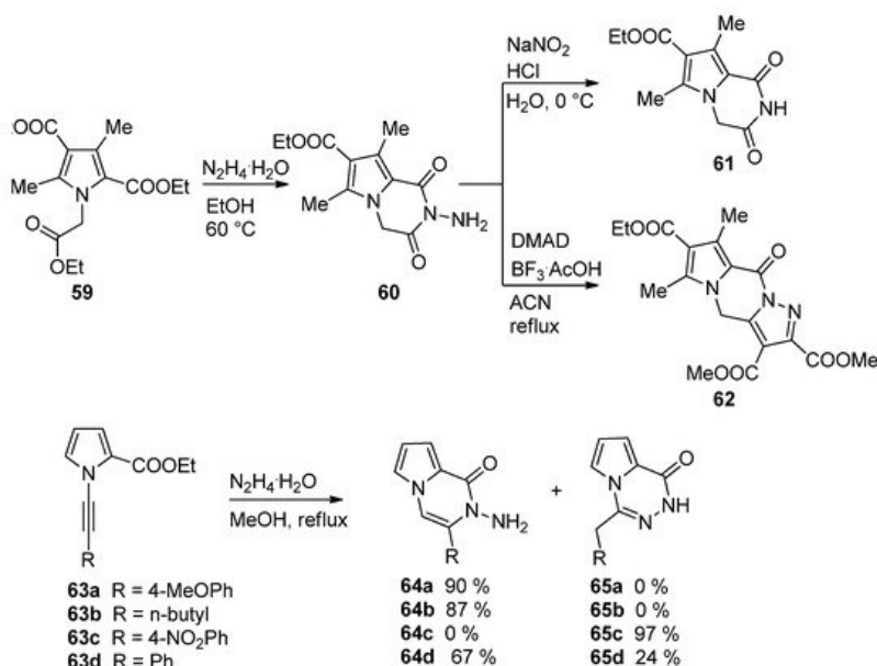
Scheme 17. Reactions of bis-electrophilic pyrroles with hydrazine.
