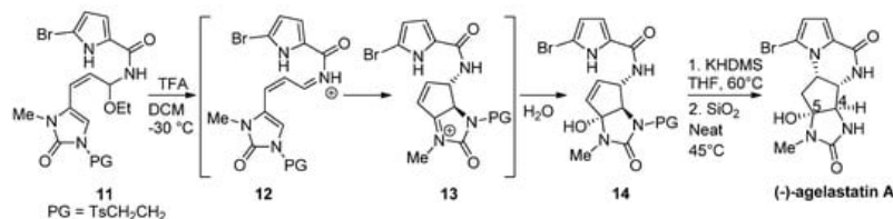
Scheme 3. Silica-promoted synthesis of (-)-agelastatin A.
