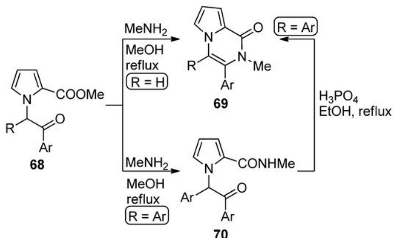
Scheme 19. Cyclization of N -phenacylpyrroles and methylamine.
