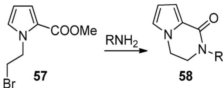
Scheme 16. Bromine substitution and lactamization with primary amines.
