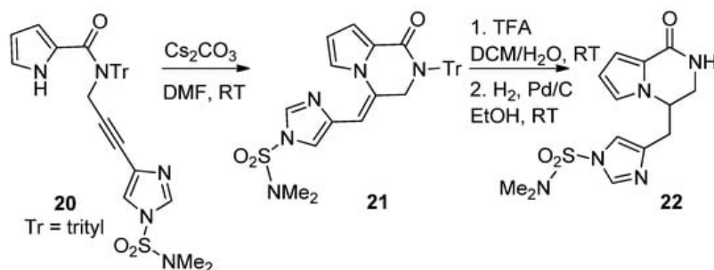
Scheme 5. Base-catalyzed ring closure of N -propargyl pyrrole-carboxamides.
