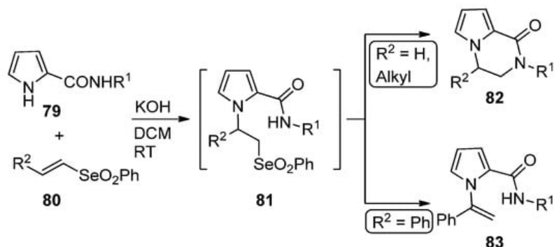
Scheme 22. Domino reaction of pyrrole-2-carboxamides and vinyl selenones.
