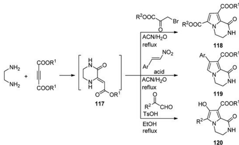
Scheme 32. Three-component reactions leading to dihydropyrrolopyrazinones.
