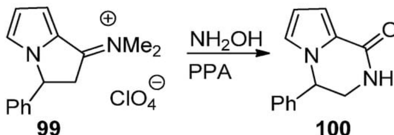
Scheme 27. Ring expansion of pyrrolizidine to pyrrolopyrazinone.
