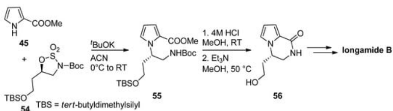
Scheme 15. Boc-strategy toward longamide B derivatives.
