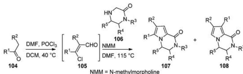
Scheme 29. Two-step synthesis of pyrrolopyrazinones from 2-chloroacroleins.
