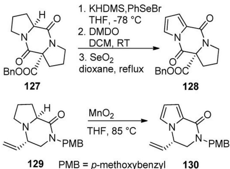
Scheme 35. Aromatization of pyrrolidino-fused diketopiperazines and pyrazinones.
