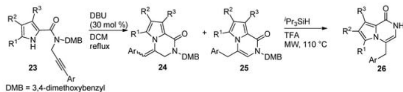
Scheme 6. Ring closure of N -(3-arylpropargyl) pyrrole-carboxamides.
