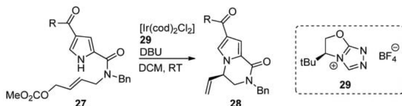
Scheme 7. Iridium-catalyzed intramolecular allylation strategy toward pyrrolopyrazinones.
