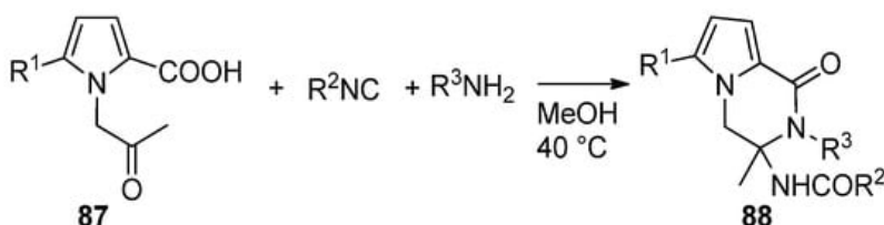
Scheme 24. Ugi reaction toward pyrrolopyrazinones.
