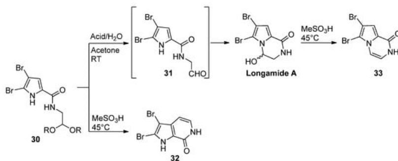
Scheme 8. Alternate intramolecular reactions of acetals and pyrrole.
