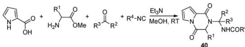
Scheme 11. Pyrrolopyrazinones by Ugi four component reaction.
