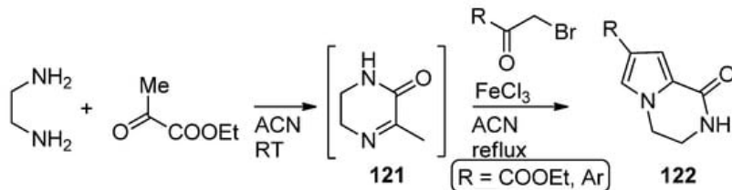
Scheme 33. Three-component reaction with ethyl pyruvate.
