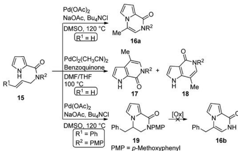
Scheme 4. Palladium-catalyzed cyclization of N -allyl pyrrole-2-carboxamide.
