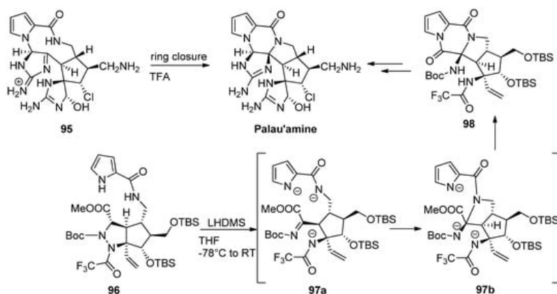
Scheme 26. Different cyclization strategies to palau'amine.
