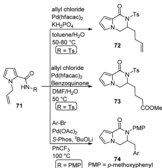
Scheme 20. Pd(II)-catalyzed carboamination reactions.
