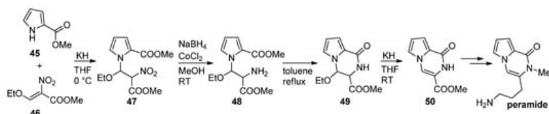
Scheme 13. First total synthesis of peramide.
