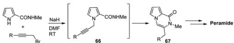
Scheme 18. N -propargylpyrrole-2-carboxamide synthesis and cyclization.
