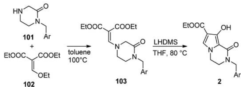
Scheme 28. Synthesis of hydroxy-substituted pyrrolopyrazinones.
