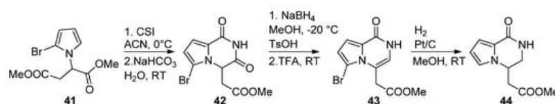
Scheme 12. Cyclization of 1-monosubstituted pyrrole with CSI.
