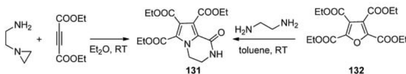
Scheme 36. Formation of pyrrolopyrazinone triesters.
