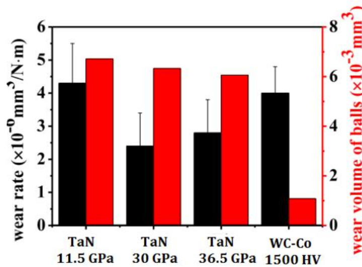
Figure 18. Wear rate of 2.5–3 \mu\text{m} thick TaN coatings deposited on WC-Co substrate using the reactive magnetron sputtering technique, and wear volume of steel balls, reprinted from Tribology International , Reference [134], with permission from Elsevier.
