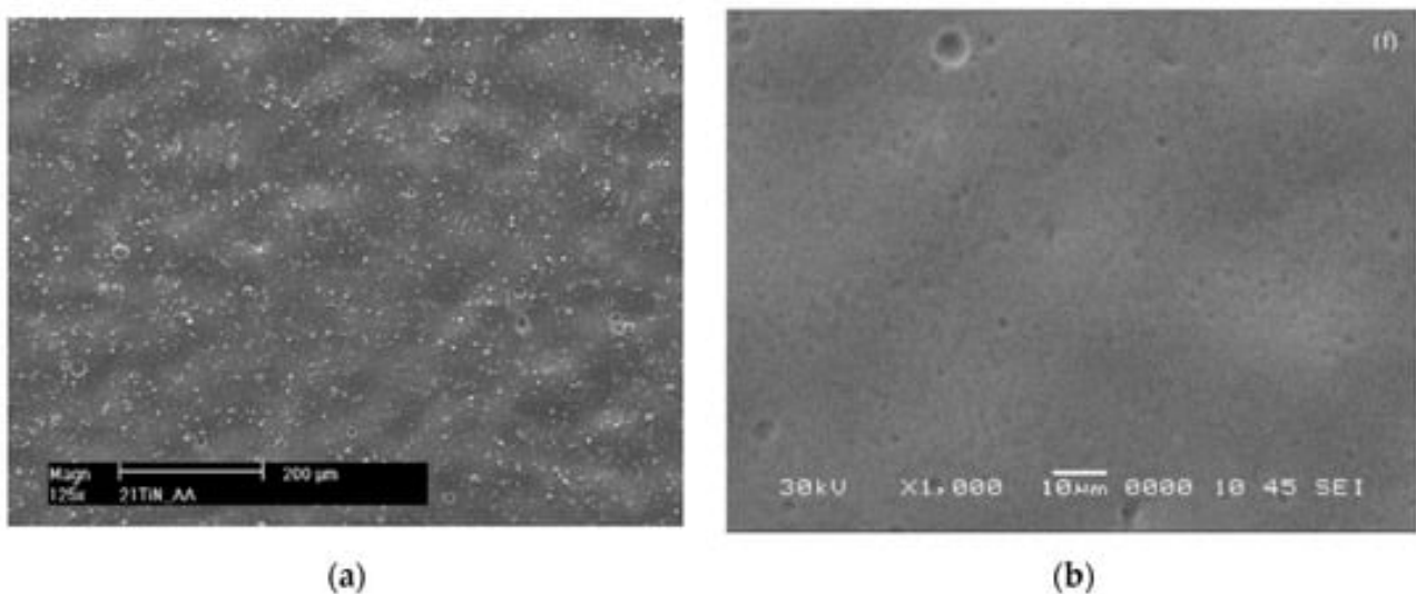
Figure 6. Undulation of (a) 3.6 μm thick TiN coating deposited on X6CrNiTi18-10 steel by means of a cathodic arc evaporation physical vapor deposition (PVD) method, reprinted from Engineering Failure Analysis , Reference [94],
