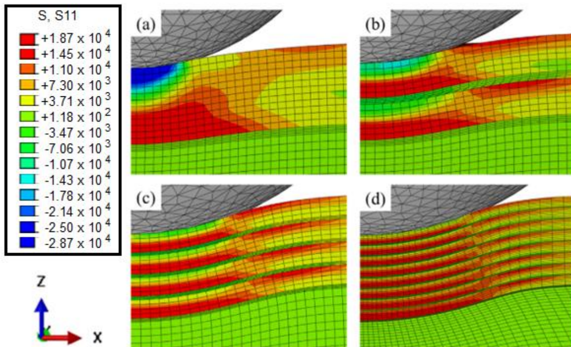
Figure 12. Stress fields in the 16 \mu\text{m} TiN coating (a) and the 16 \mu\text{m} TiN/Ti multilayer coatings with the bilayers number of (b) N = 2 , (c) N = 4 and (d) N = 8 deposited on Ti-6Al-4V alloy by combining the techniques of a filtered cathode vacuum arc and a metal vapor vacuum arc ion implantation, reprinted from Surface and Coatings Technology , Reference [16], with permission from Elsevier.
