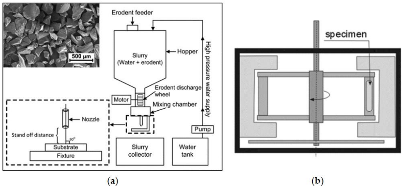
Figure 9. The examples of (a) a jet type apparatus, reprinted from Wear , Reference [108], with permission from Elsevier and (b) a slurry pot, reprinted from Engineering Failure Analysis , Reference [109], with permission from Elsevier.
