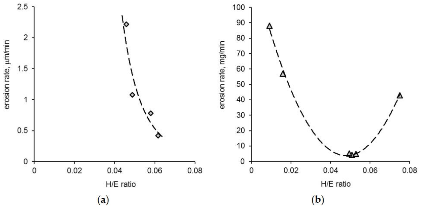
Figure 15. Relation between H/E ratio and erosion rate of various PVD coatings, performed on the basis of on data from (a) Reference [120], (b) Reference [110].
