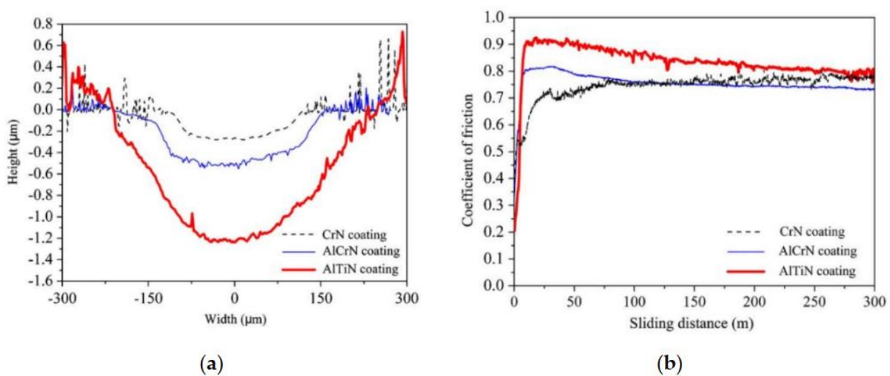
Figure 17. Wear track profiles (a) and coefficients of friction (b) of the 2 μm thick CrN, 1 μm thick AlCrN and 2 μm thick AlTiN coatings deposited on cemented carbide (10 wt.% Co and 90 wt.% WC) using the multi-arc ion plating technique, after the entire tests performed at the normal load of 5 N; the sliding velocities of 10m/min; the wear track nominal diameter of 10 mm; the total sliding distance of 300 m, using a Si 3 N 4 ball with diameter of 4mm, surface roughness Ra of 0.02 μm and hardness of HV1600 as the counterpart, reprinted from Tribology International , Reference [133], with permission from Elsevier.
