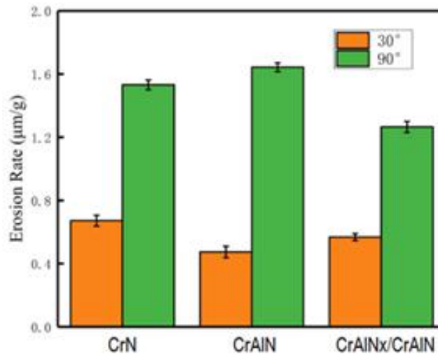
Figure 14. Erosion rate of 2.24 µm thick CrN, 1.92 µm thick CrAlN and 2.17 µm thick CrAlNx/CrAlN coatings deposited on TC11 titanium alloy using the arc ion plating technique, reprinted from Vacuum , Reference [9], with permission from Elsevier.
