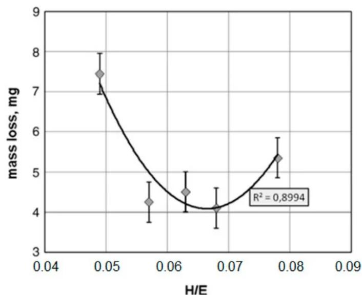
Figure 7. Correlation between H/E ratio and mass loss in cavitation tests of 4 \mu\text{m} thick TiN coatings deposited on X6CrNiTi18-10 steel by means of a cathodic arc evaporation PVD method, reprinted from Surface and Coatings Technology , Reference [92], with permission from Elsevier.
