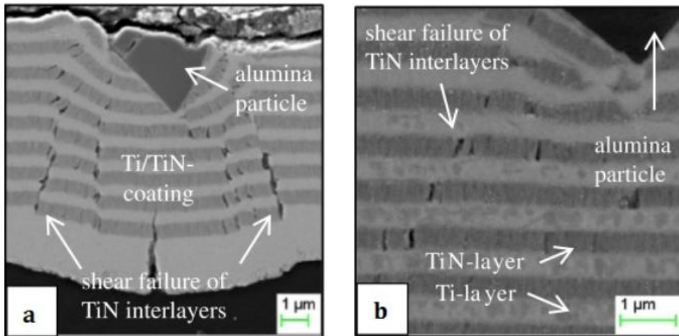
Figure 10. Shear fracture in TiN/Ti coatings with a thickness of (a) 10 μm and (b) 30 μm deposited on polymer matrix composite by means of a magnetron sputtering method, reprinted from Wear , Reference [118], with permission from Elsevier.
