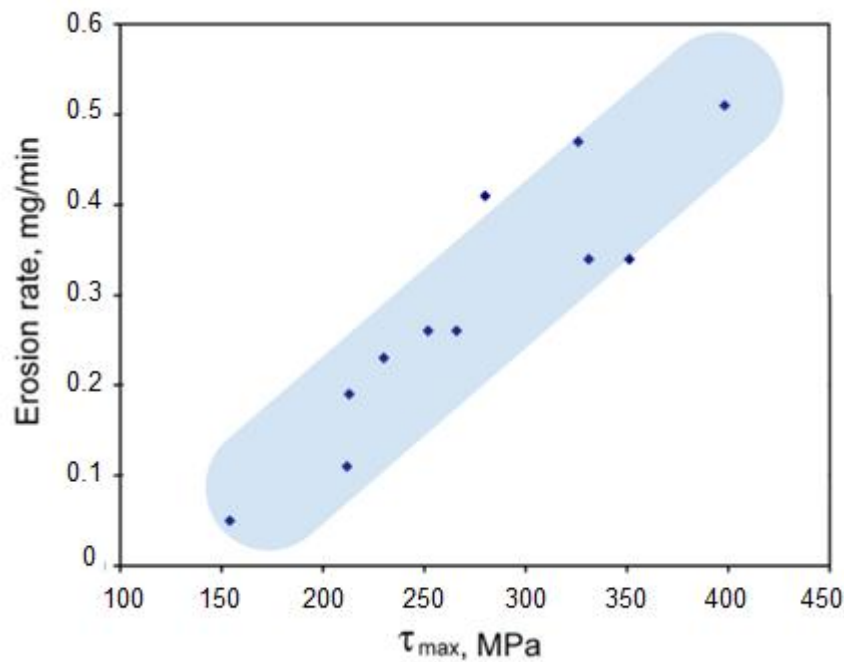
Figure 11. Correlation between erosion rate and maximum shear stress in Ti/TiN and Ti/Ti(V,Zr)N multilayered coatings with thickness from 5 to 20 \mu\text{m} deposited on Ti-6Al-4V alloy by the Arc-PVD method, reprinted from Wear , Reference [22], with permission from Elsevier.
