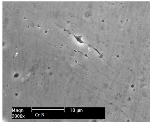
Figure 5. Development of a crack thorough pinholes in 4 μm thick Cr-N coating deposited on X6CrNiTi18-10 austenitic steel by means of a cathodic arc evaporation method (own investigations).
