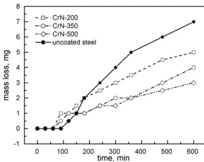
Figure 3. Cavitation curves of 3.7 \mu\text{m} thick Cr-N coatings deposited on X6CrNiTi18-10 stainless steel by means of the cathodic arc evaporation method and uncoated stainless steel reprinted from Wear , Reference [79], with permission from Elsevier.
